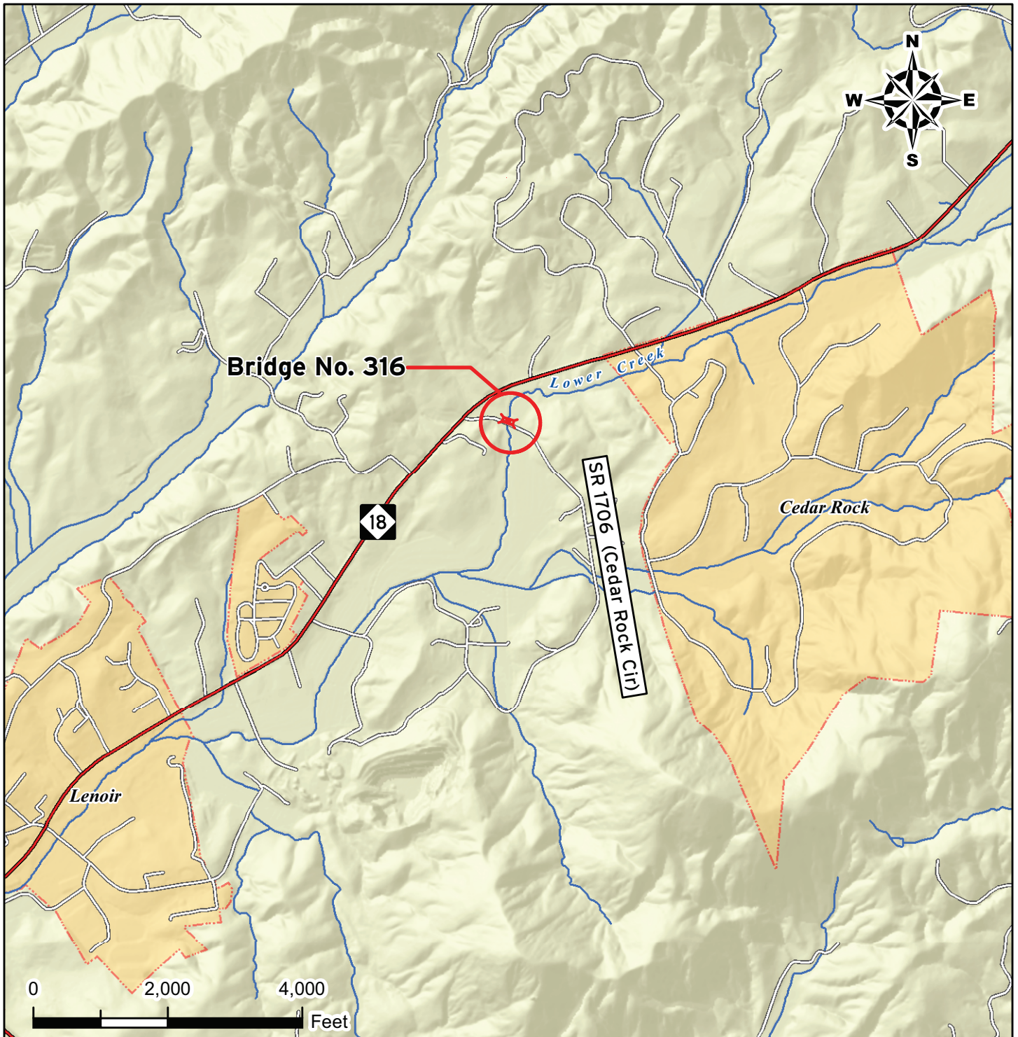
NCDOT Division of Highways Division 11 Low Impact Bridge Replacements Bridge Location Map Bridge No. 316 SR 1706 over Lower Creek Caldwell County July 2012 Figure 1
